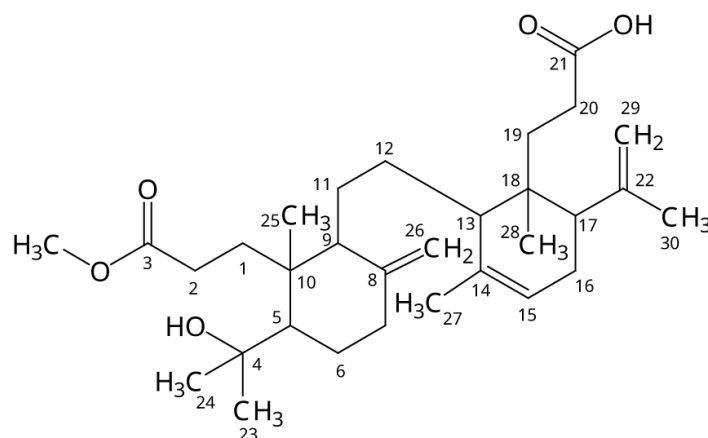
Figure 2. Isolated compound 1, Lamesticum A.
