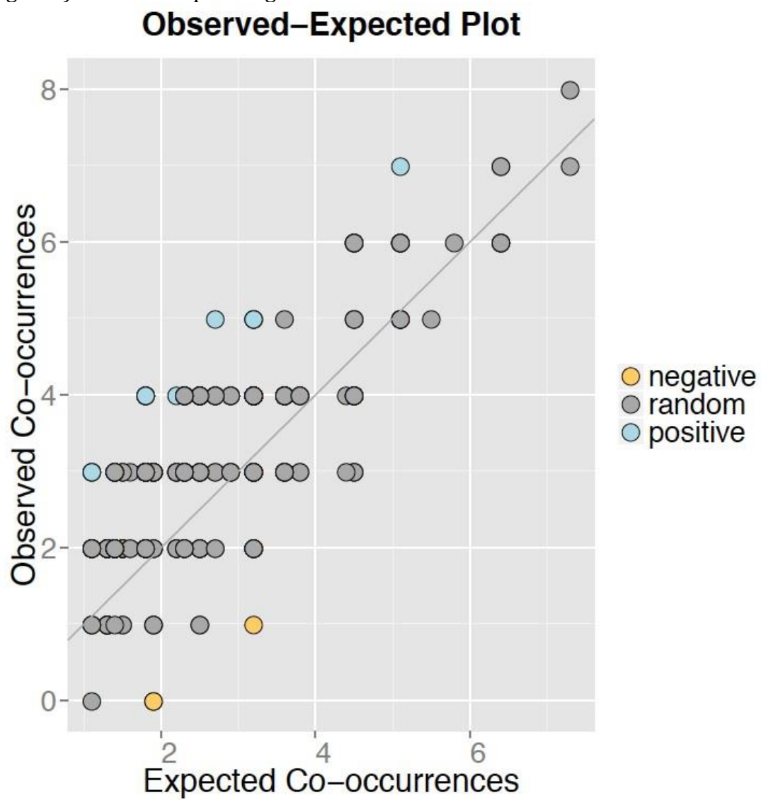
Fig. S1n) Paired OTU plot stage 80
