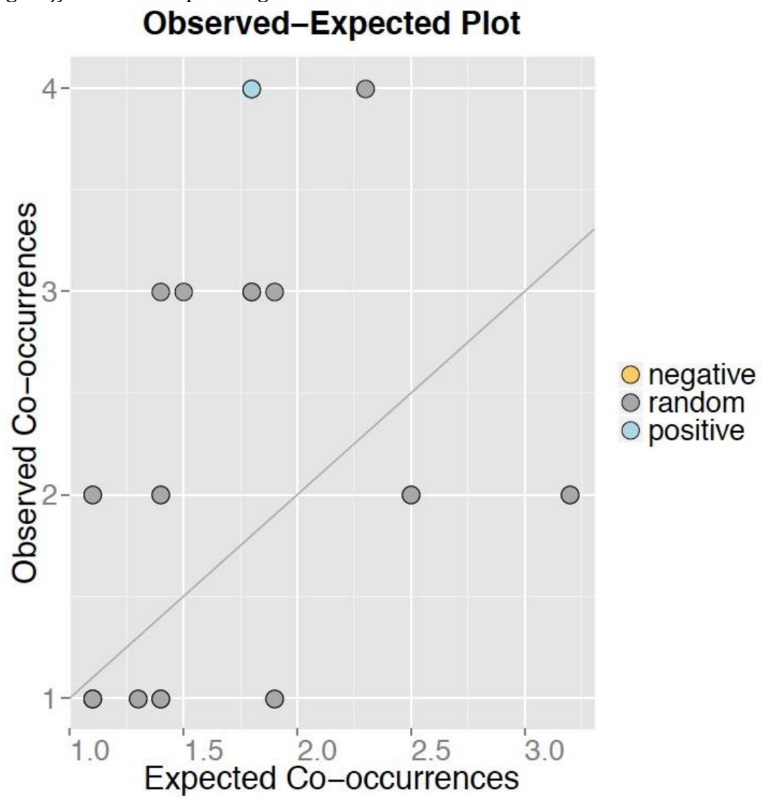
Fig. S1j) Paired OTU plot stage 48
