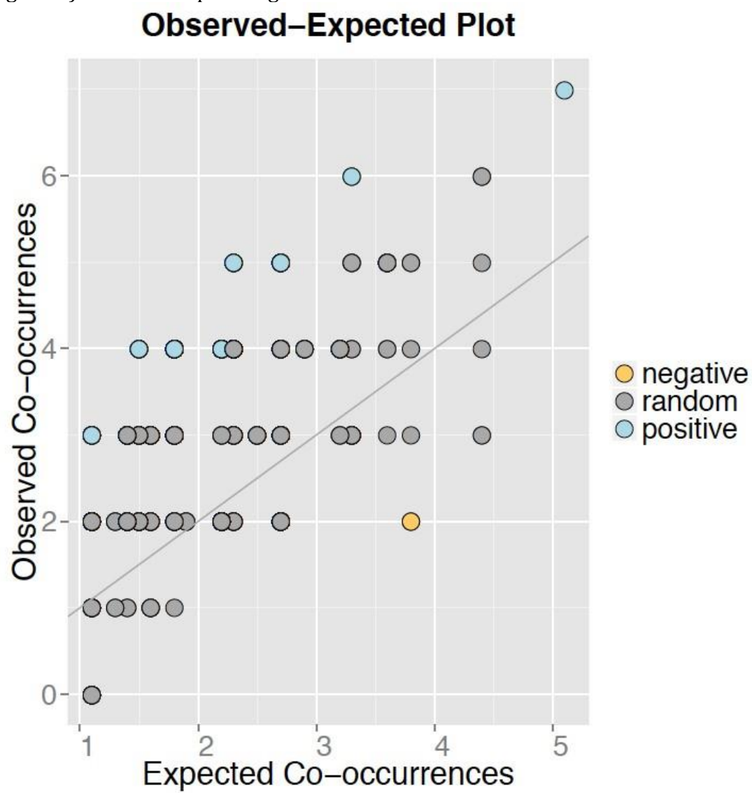
Fig. S1m) Paired OTU plot stage 72
