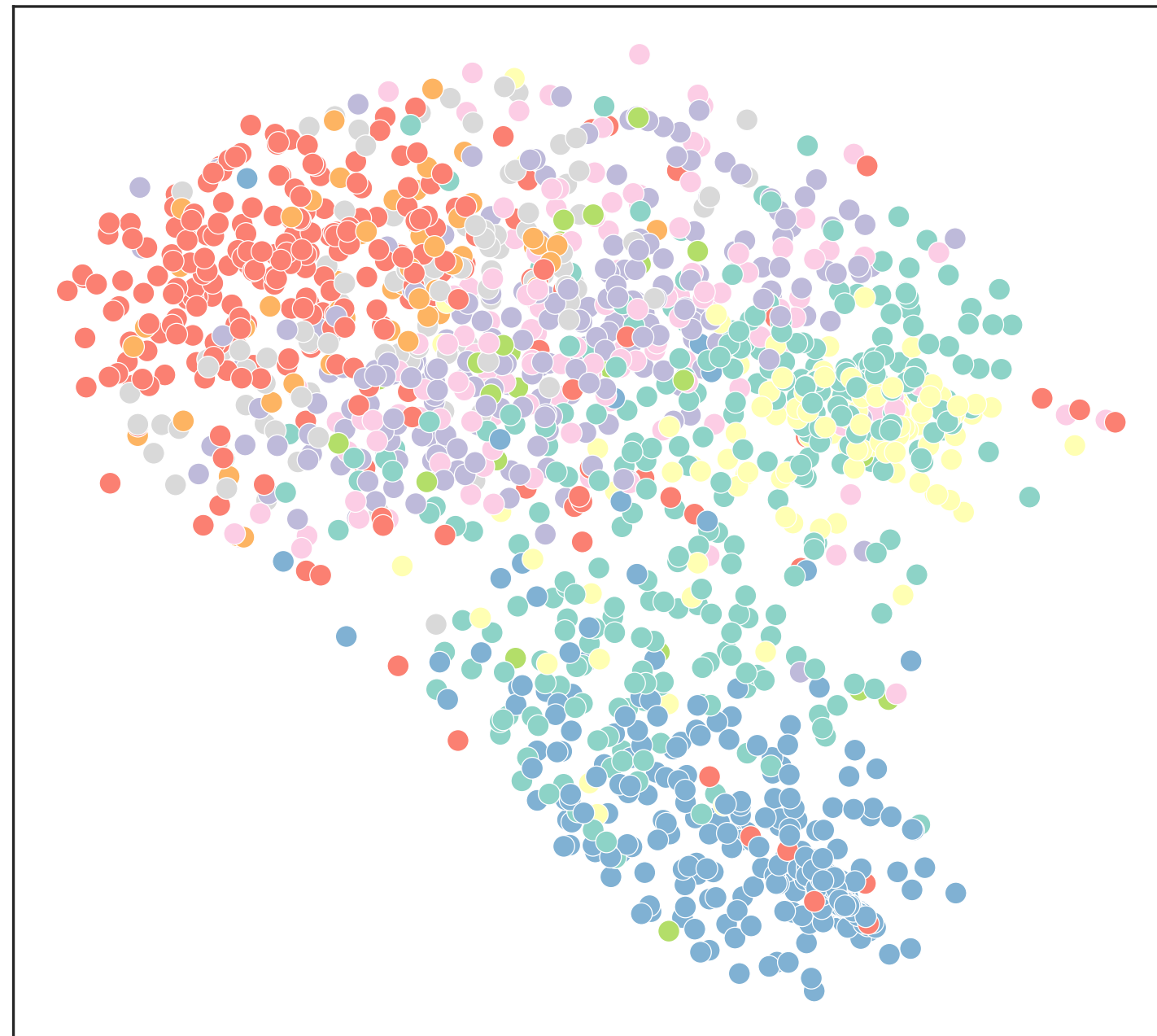
netsmooth
