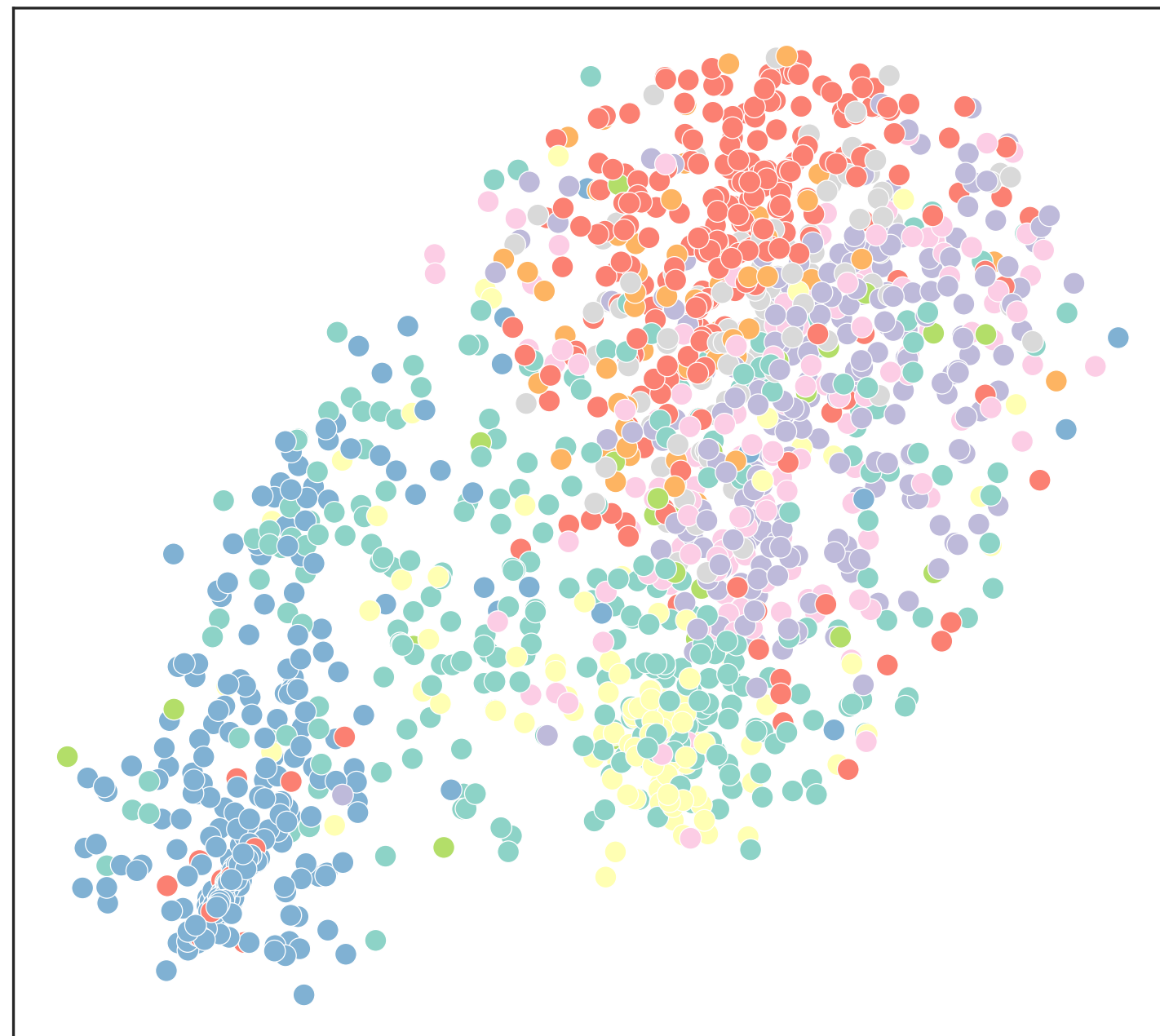
scImpute
